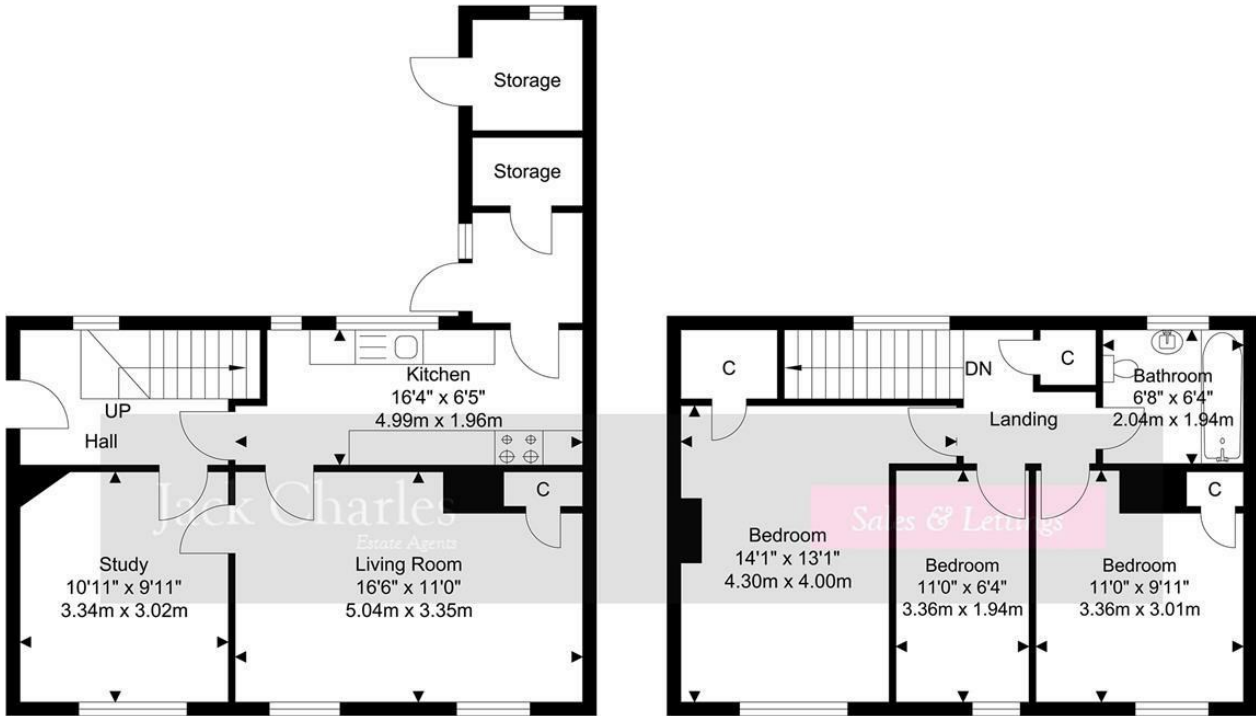
Ground Floor Approximate Floor Area 551.75 SQ.FT. (51.26 SQ.M.)
