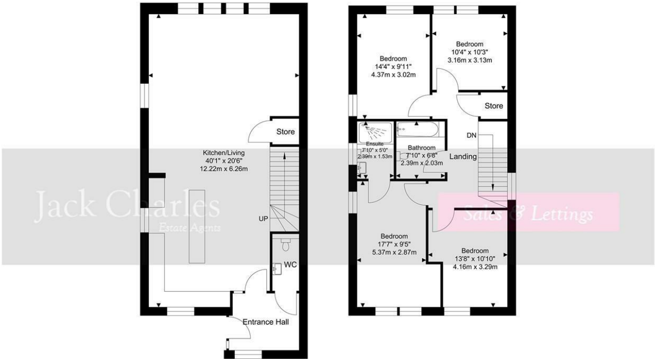
Ground Floor Approximate Floor Area 877.25 SQ.FT. (81.50 SQ.M.)
