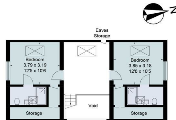
Outbuilding - First Floor
