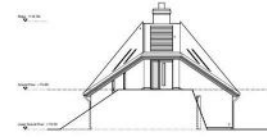
South West (Front) Elevation
