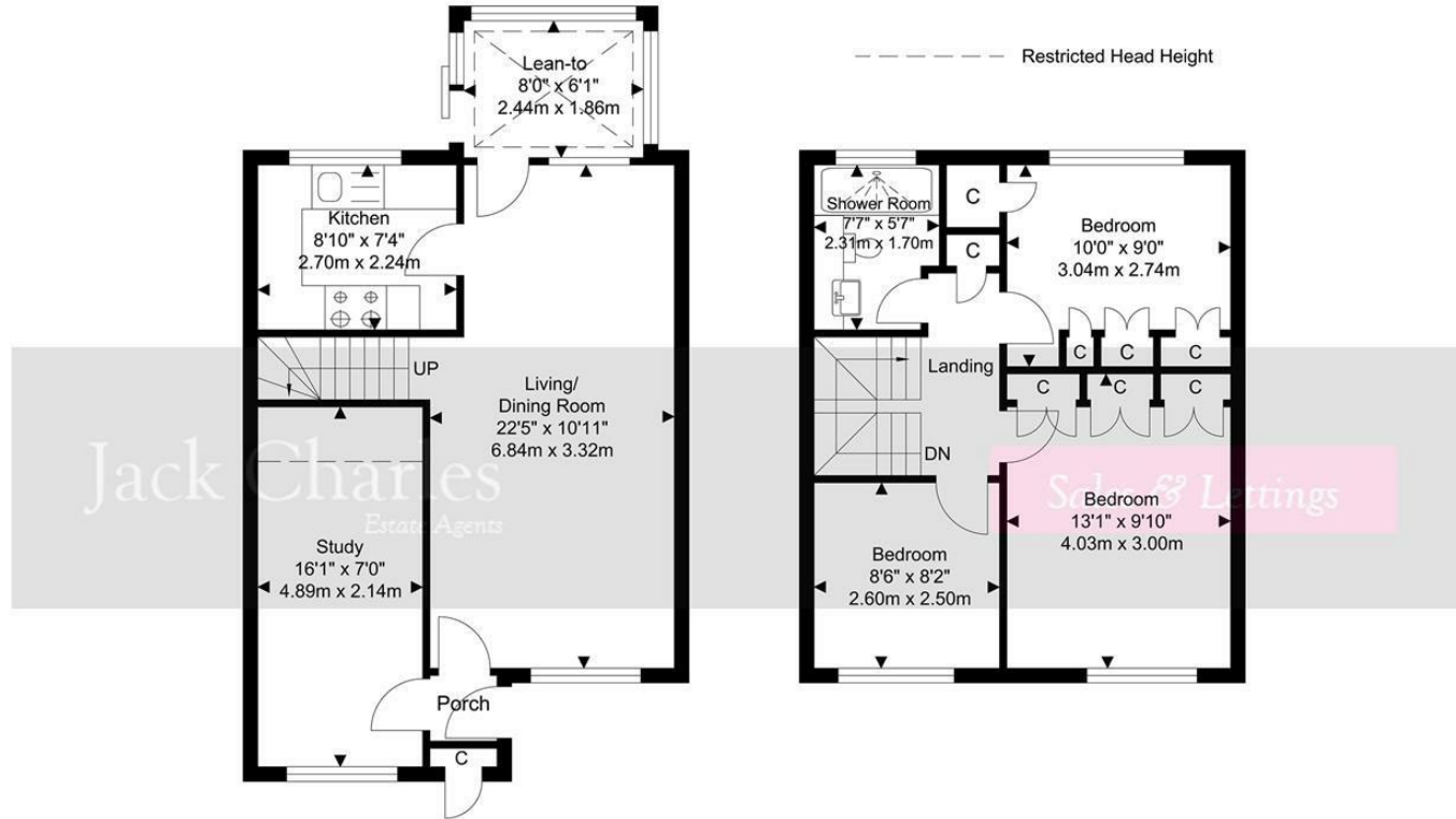
Ground Floor Approximate Floor Area 515.05 SQ.FT. (47.85 SQ.M.)
