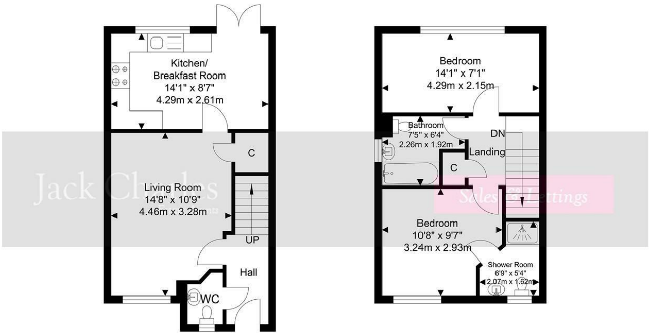
Ground Floor Approximate Floor Area 349.61 SQ.FT. (32.48 SQ.M.)
